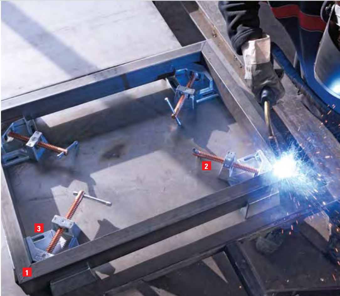
Angle clamps (WSM)
